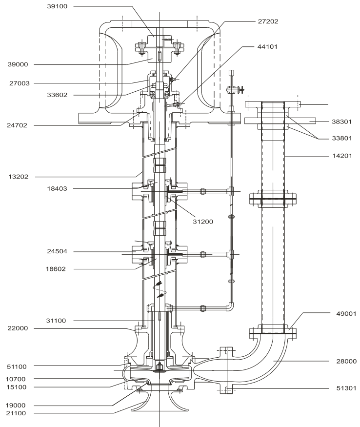
SHS PUMP TYPICAL DRAWING
